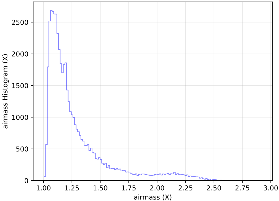
too_elab_heavy_r128_d3_griz_v3.4_10yrs Yr 1 r band: airmass Histogram
