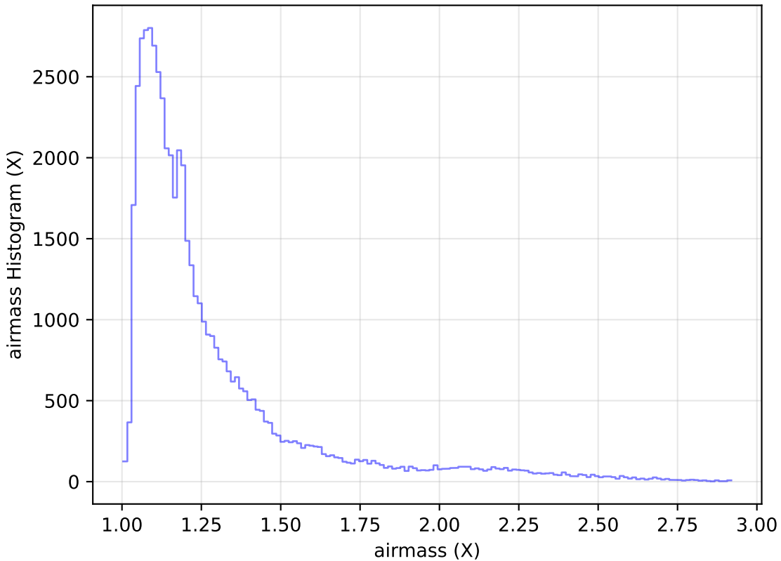
too_elab_heavy_r128_d3_griz_v3.4_10yrs Yr 1 i band: airmass Histogram
