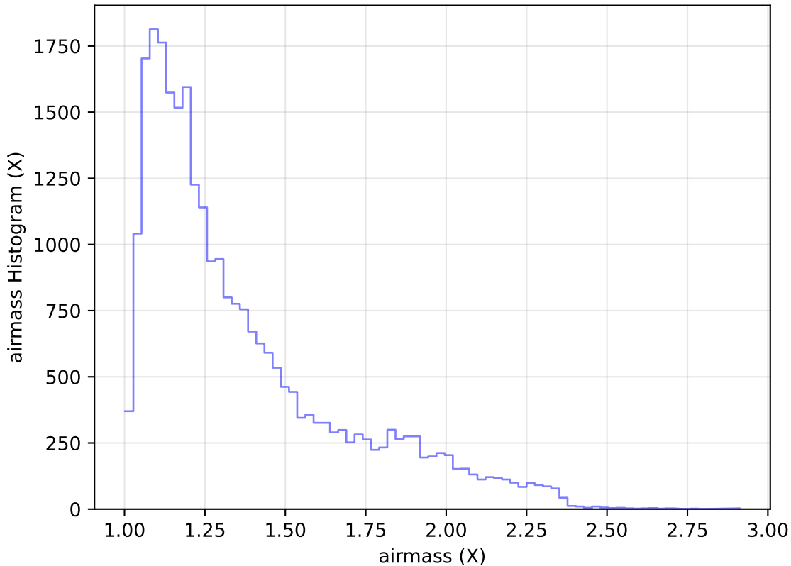
too_elab_heavy_r128_d3_griz_v3.4_10yrs Yr 1 g band: airmass Histogram
