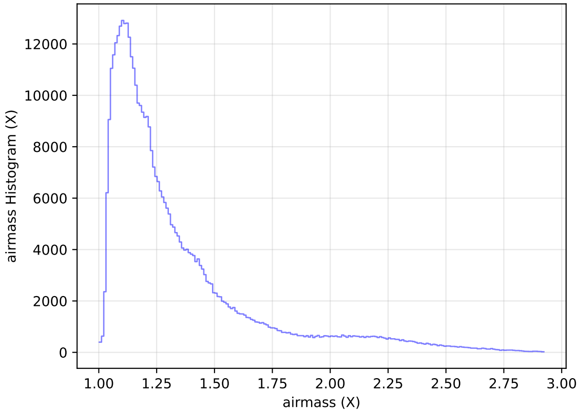
too_elab_heavy_r128_d3_griz_v3.4_10yrs WFD z band: airmass Histogram
