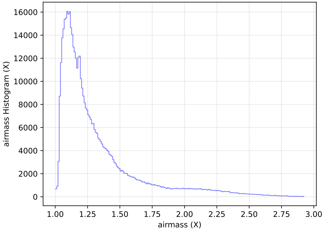
too_elab_heavy_r128_d3_griz_v3.4_10yrs WFD i band: airmass Histogram
