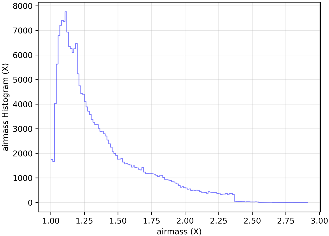
too_elab_heavy_r128_d3_griz_v3.4_10yrs WFD g band: airmass Histogram
