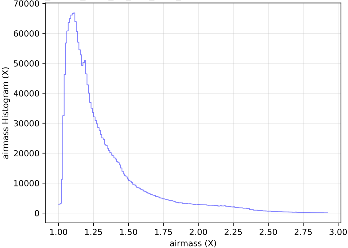
too_elab_heavy_r128_d3_griz_v3.4_10yrs WFD all bands: airmass Histogram
