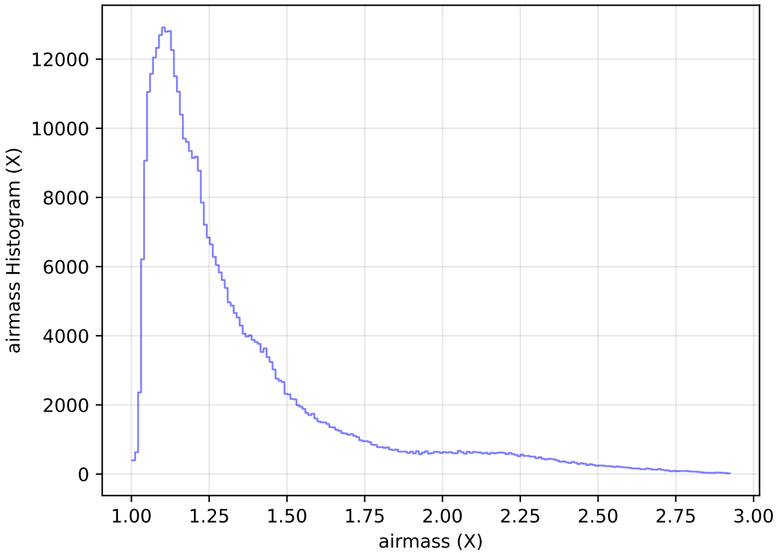
too_elab_heavy_r128_d3_griz_v3.4_10yrs All sky z band: airmass Histogram
