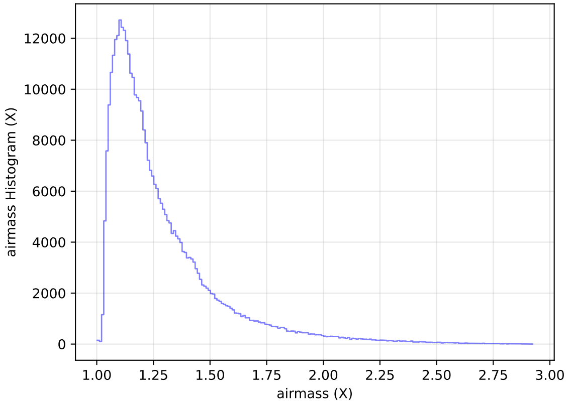
too_elab_heavy_r128_d3_griz_v3.4_10yrs All sky y band: airmass Histogram
