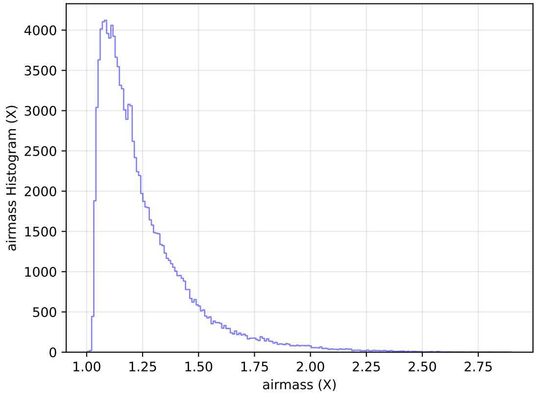
too_elab_heavy_r128_d3_griz_v3.4_10yrs All sky u band: airmass Histogram
