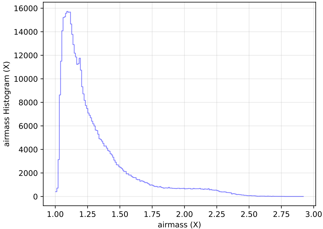
too_elab_heavy_r128_d3_griz_v3.4_10yrs All sky r band: airmass Histogram
