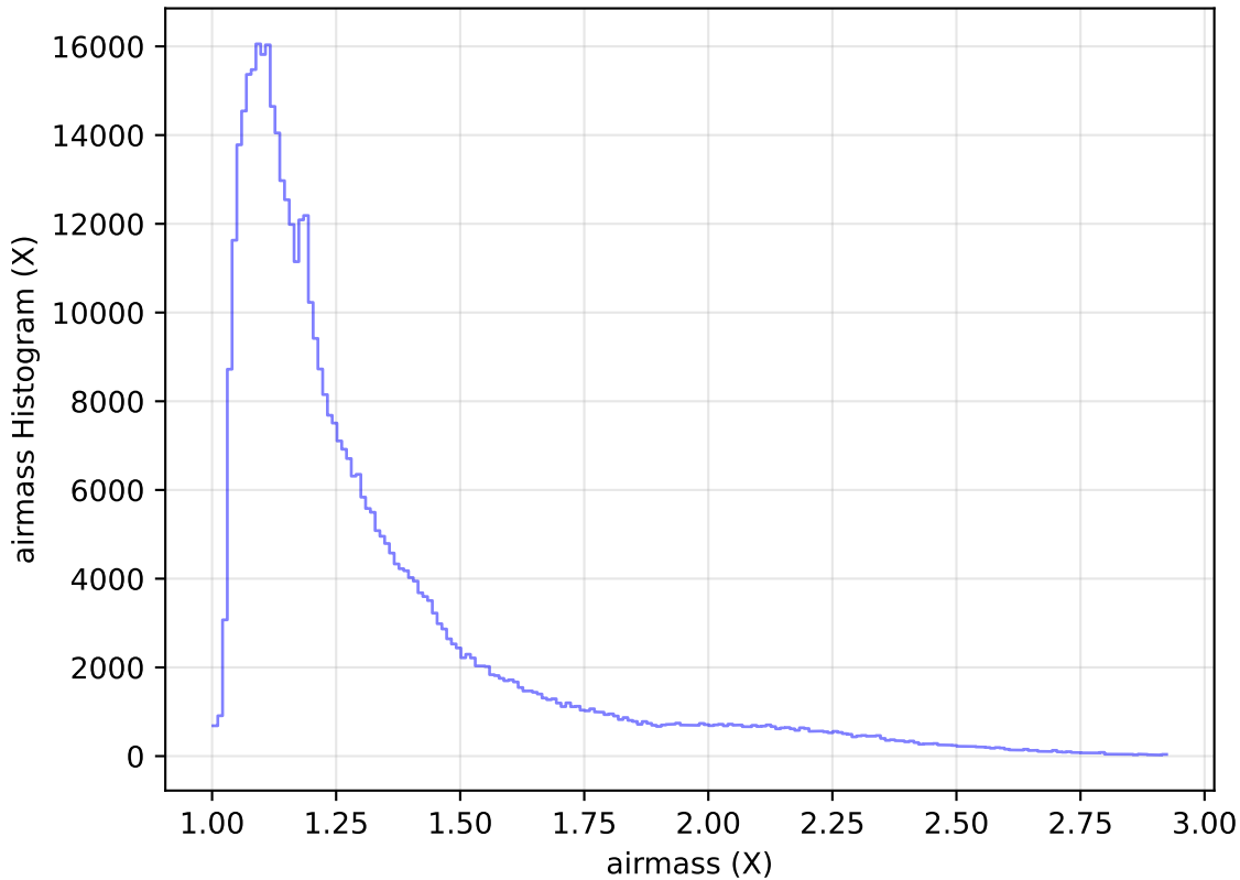
too_elab_heavy_r128_d3_griz_v3.4_10yrs All sky i band: airmass Histogram
