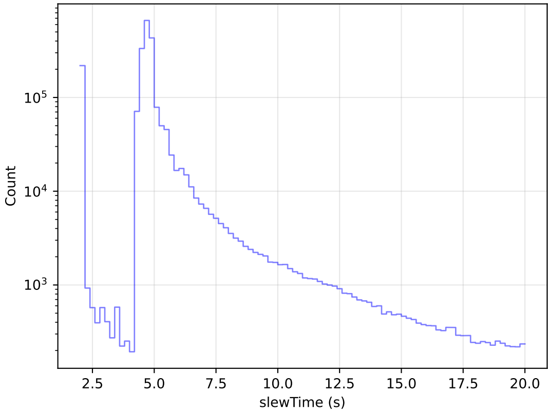
too_elab_heavy_r128_d3_griz_v3.4_10yrs All visits: Zoom Slew Time Histogram
