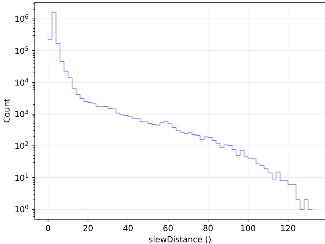
too_elab_heavy_r128_d3_griz_v3.4_10yrs All visits: Slew Distance Histogram
