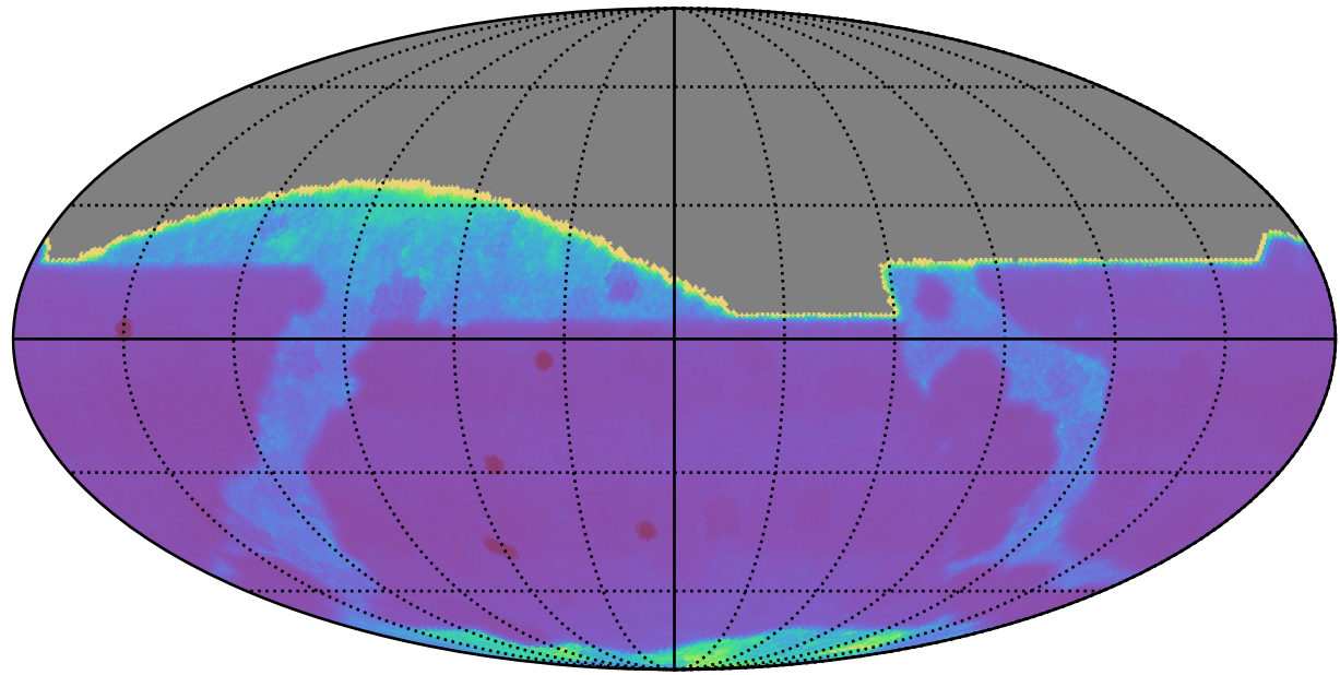
too_elab_heavy_r128_d3_griz_v3.4_10yrs All sky: Proper Motion Uncert @ 20.5
