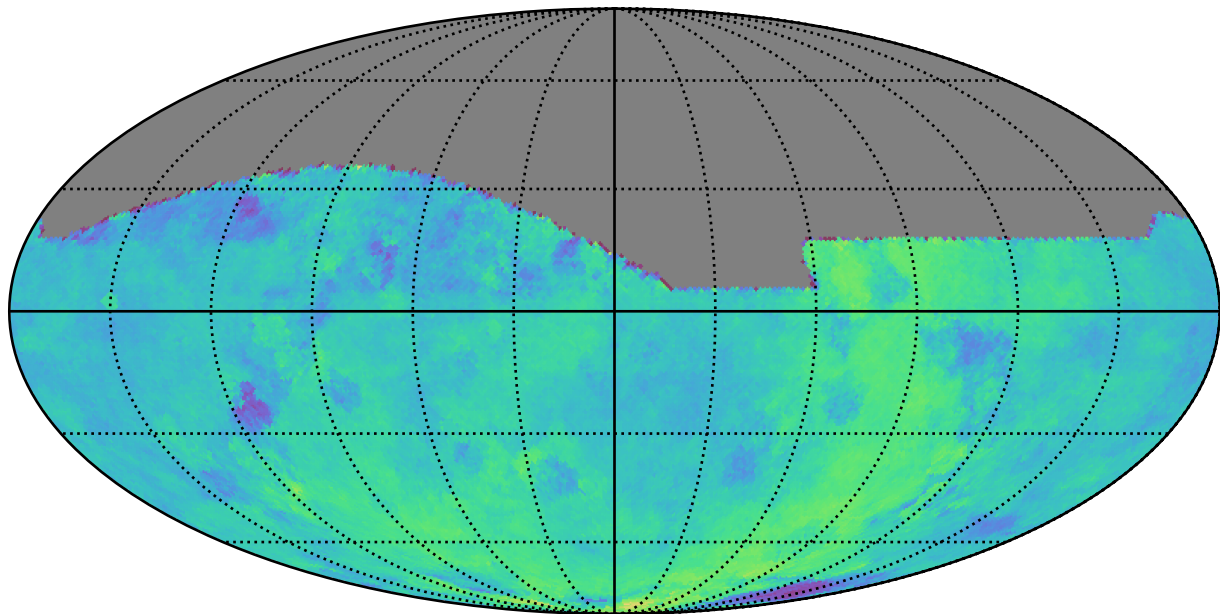
too_elab_heavy_r128_d3_griz_v3.4_10yrs All sky: Parallax Coverage @ 24.0
