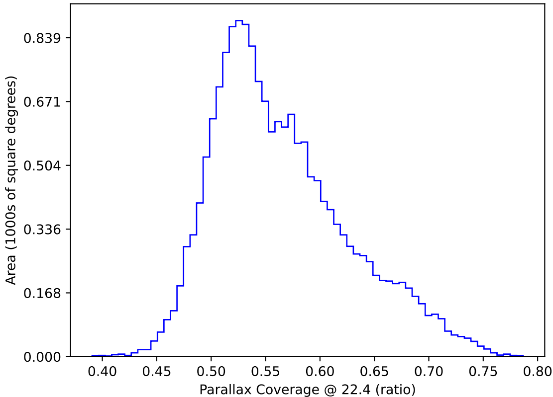
too_elab_heavy_r128_d3_griz_v3.4_10yrs WFD: Parallax Coverage @ 22.4
