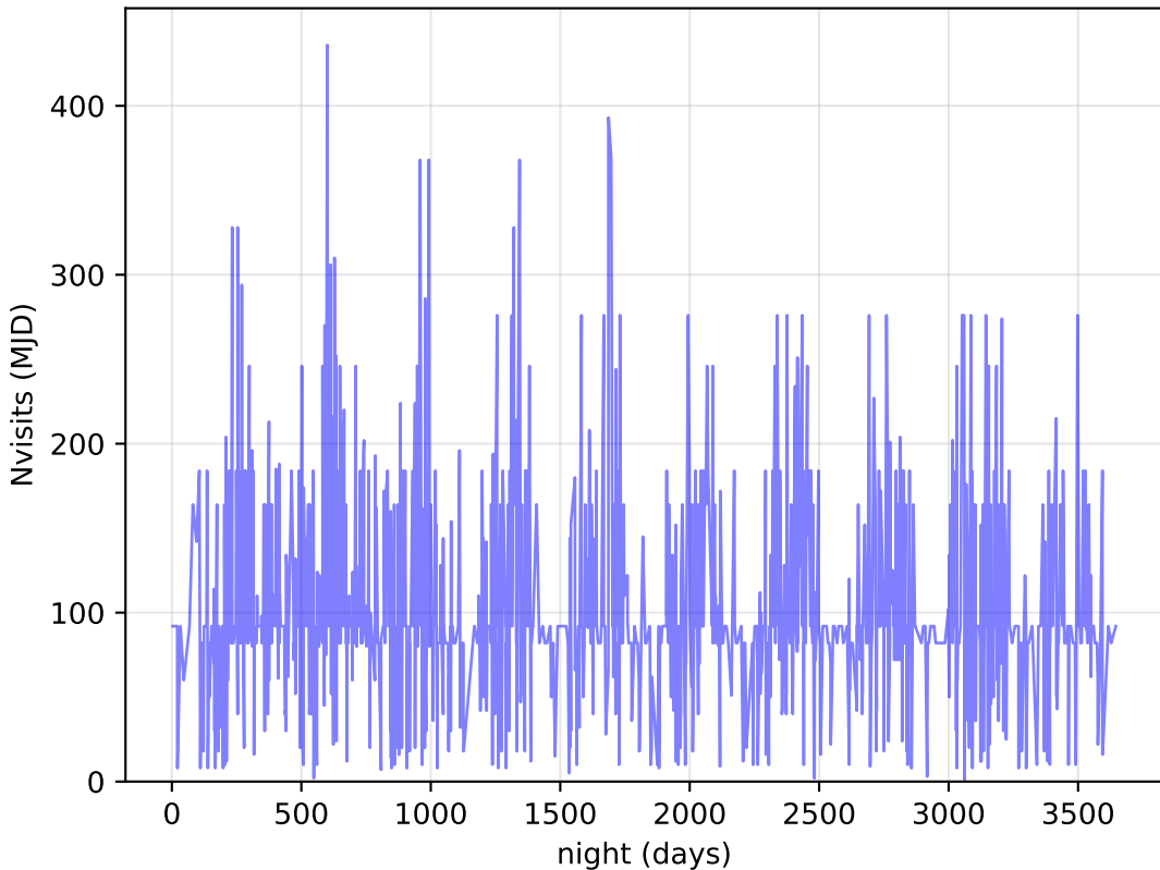
too_elab_heavy_r128_d3_griz_v3.4_10yrs DDF: Nvisits
