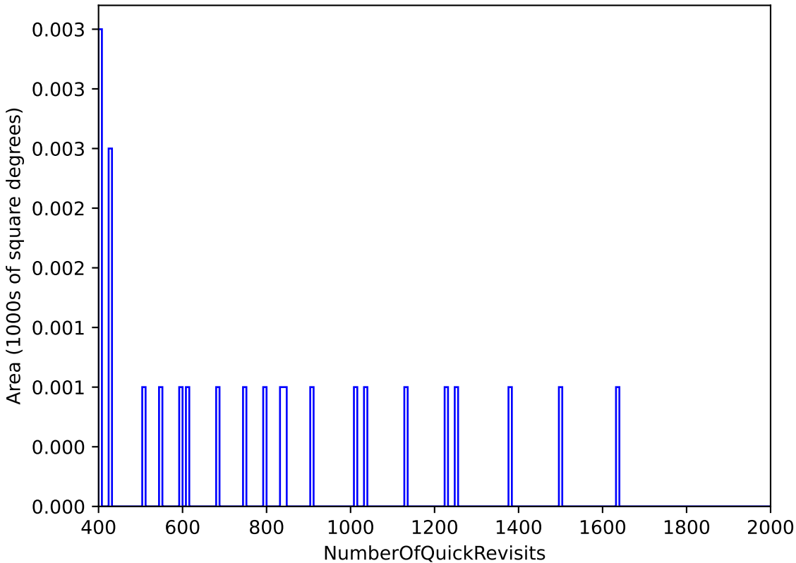
too_elab_heavy_r128_d3_griz_v3.4_10yrs WFD: NumberOfQuickRevisits
