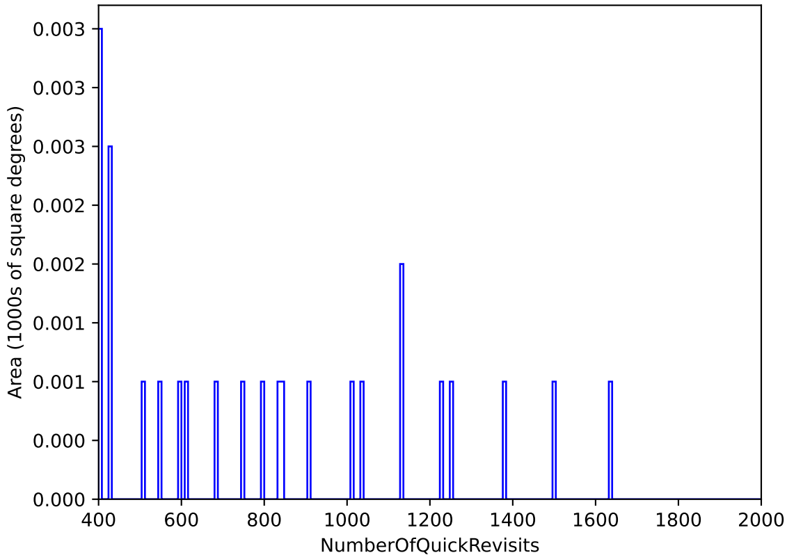
too_elab_heavy_r128_d3_griz_v3.4_10yrs All sky: NumberOfQuickRevisits
