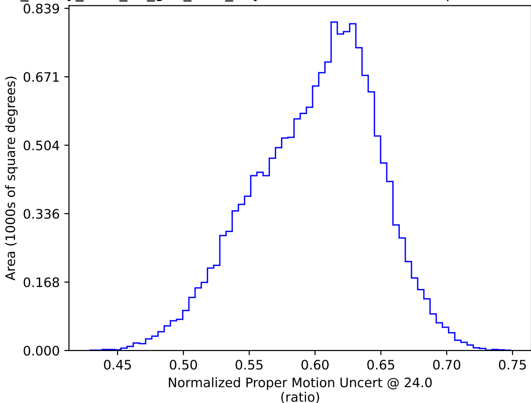
too_elab_heavy_r128_d3_griz_v3.4_10yrs WFD: Normalized Proper Motion Uncert @ 24.0
