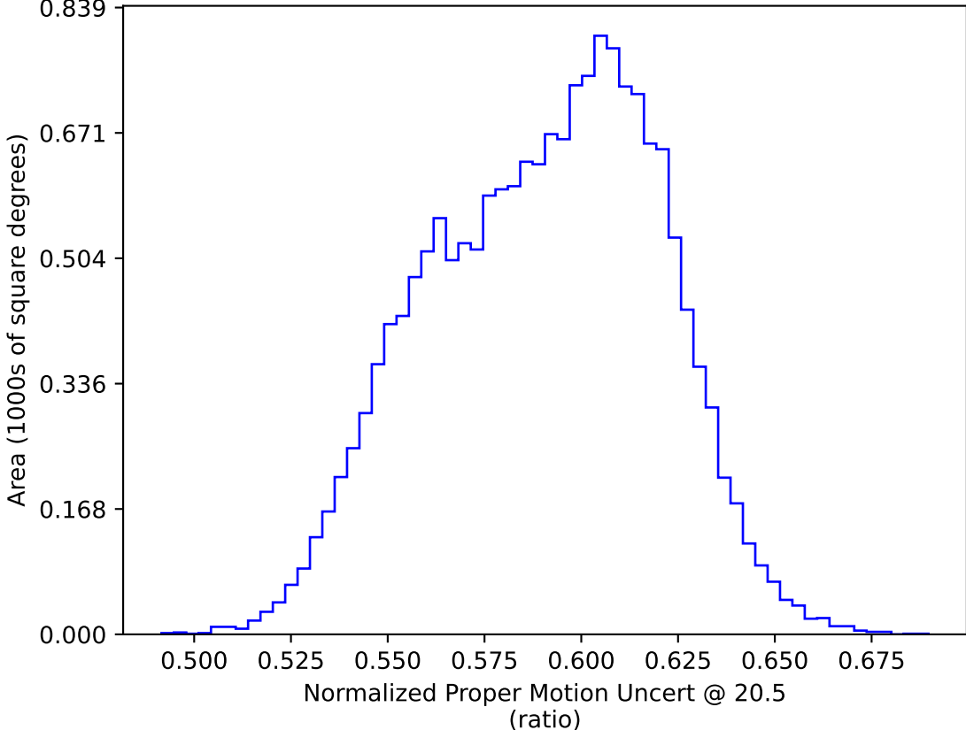
too_elab_heavy_r128_d3_griz_v3.4_10yrs WFD: Normalized Proper Motion Uncert @ 20.5
