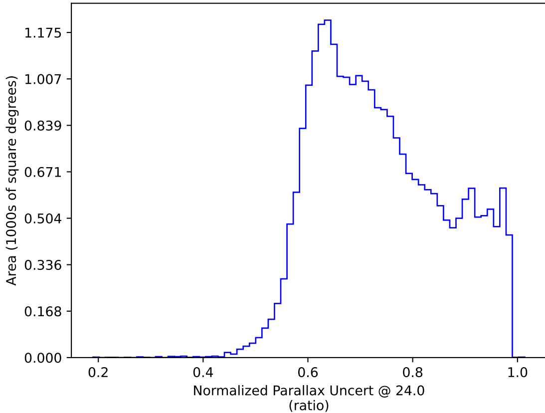
too_elab_heavy_r128_d3_griz_v3.4_10yrs All sky: Normalized Parallax Uncert @ 24.0
