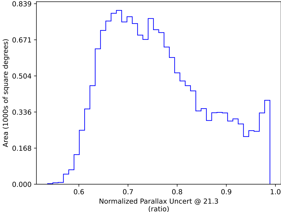
too_elab_heavy_r128_d3_griz_v3.4_10yrs WFD y band only: Normalized Parallax Uncert @ 21.3
