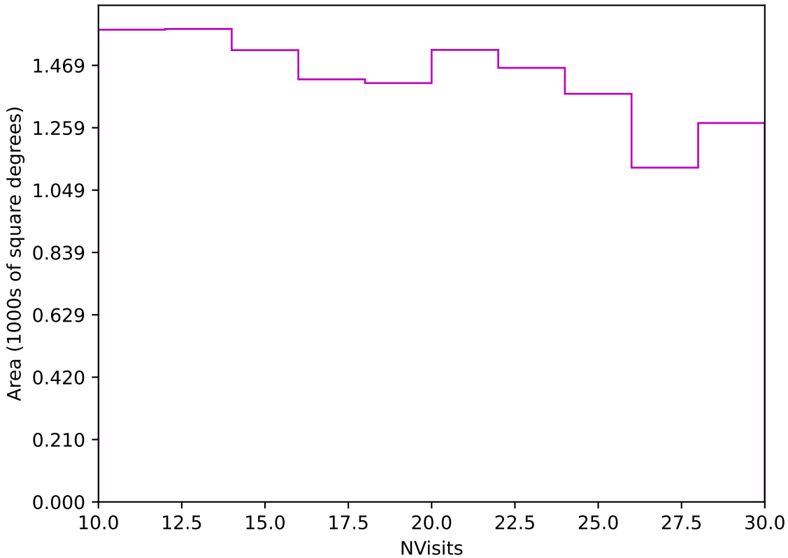
too_elab_heavy_r128_d3_griz_v3.4_10yrs Yr 3-4 z band: NVisits
