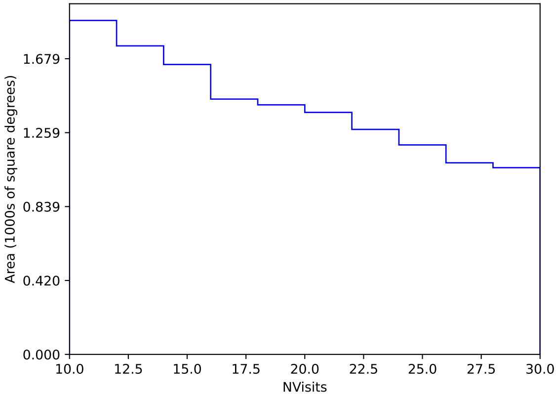
too_elab_heavy_r128_d3_griz_v3.4_10yrs Yr 3-4 y band: NVisits
