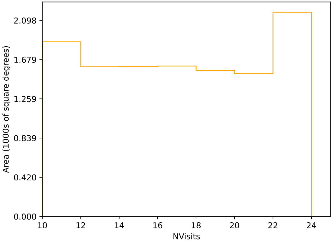
too_elab_heavy_r128_d3_griz_v3.4_10yrs Yr 3-4 r band: NVisits
