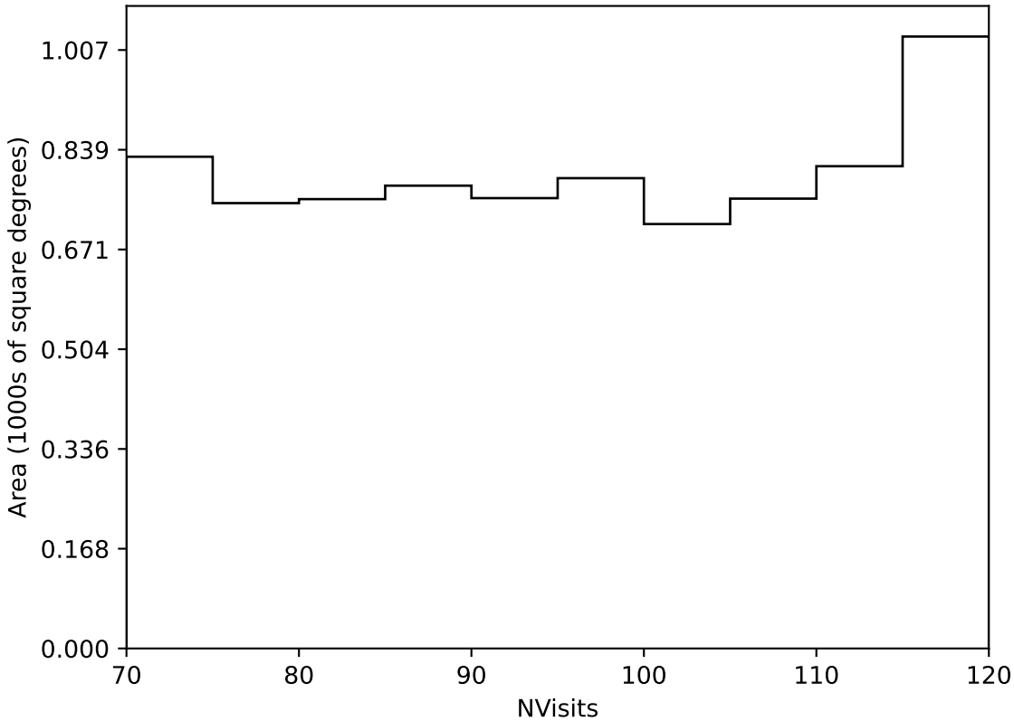
too_elab_heavy_r128_d3_griz_v3.4_10yrs Yr 3-4 all bands: NVisits
