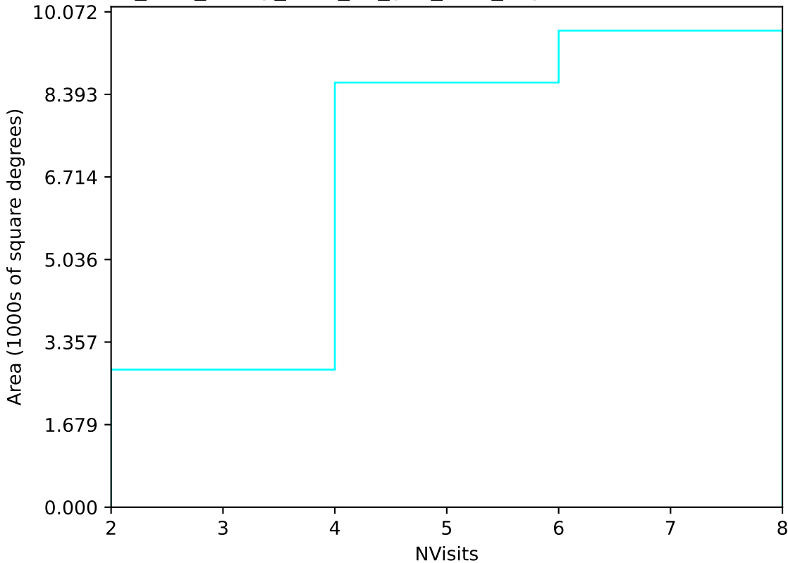
too_elab_heavy_r128_d3_griz_v3.4_10yrs Yr 1 u band: NVisits
