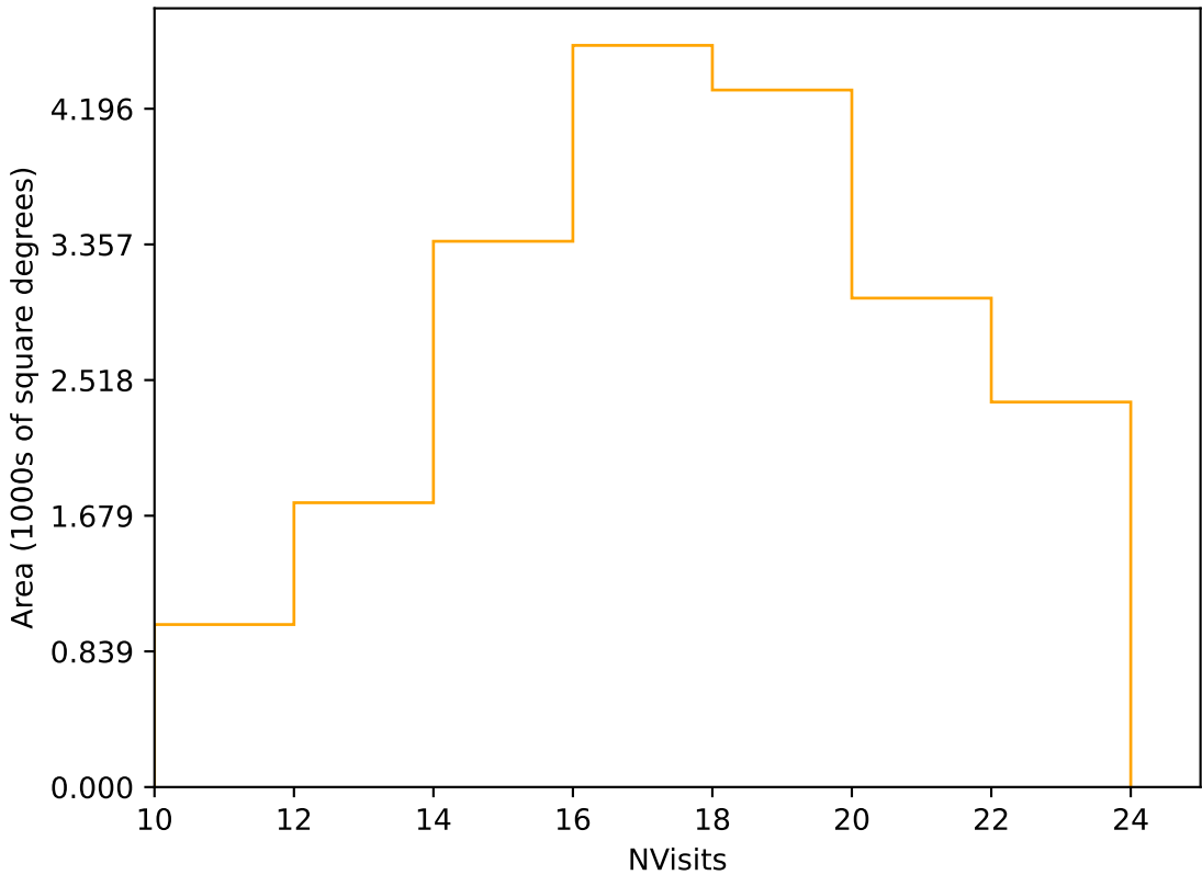
too_elab_heavy_r128_d3_griz_v3.4_10yrs Yr 1 r band: NVisits
