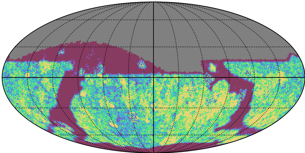
too_elab_heavy_r128_d3_griz_v3.4_10yrs Yr 1 i band: NVisits
