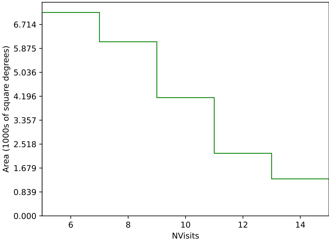
too_elab_heavy_r128_d3_griz_v3.4_10yrs Yr 1 g band: NVisits
