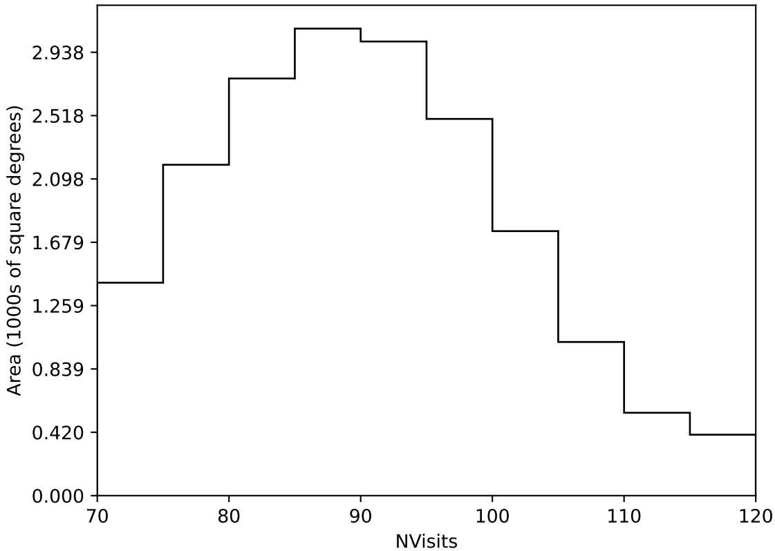
too_elab_heavy_r128_d3_griz_v3.4_10yrs Yr 1 all bands: NVisits
