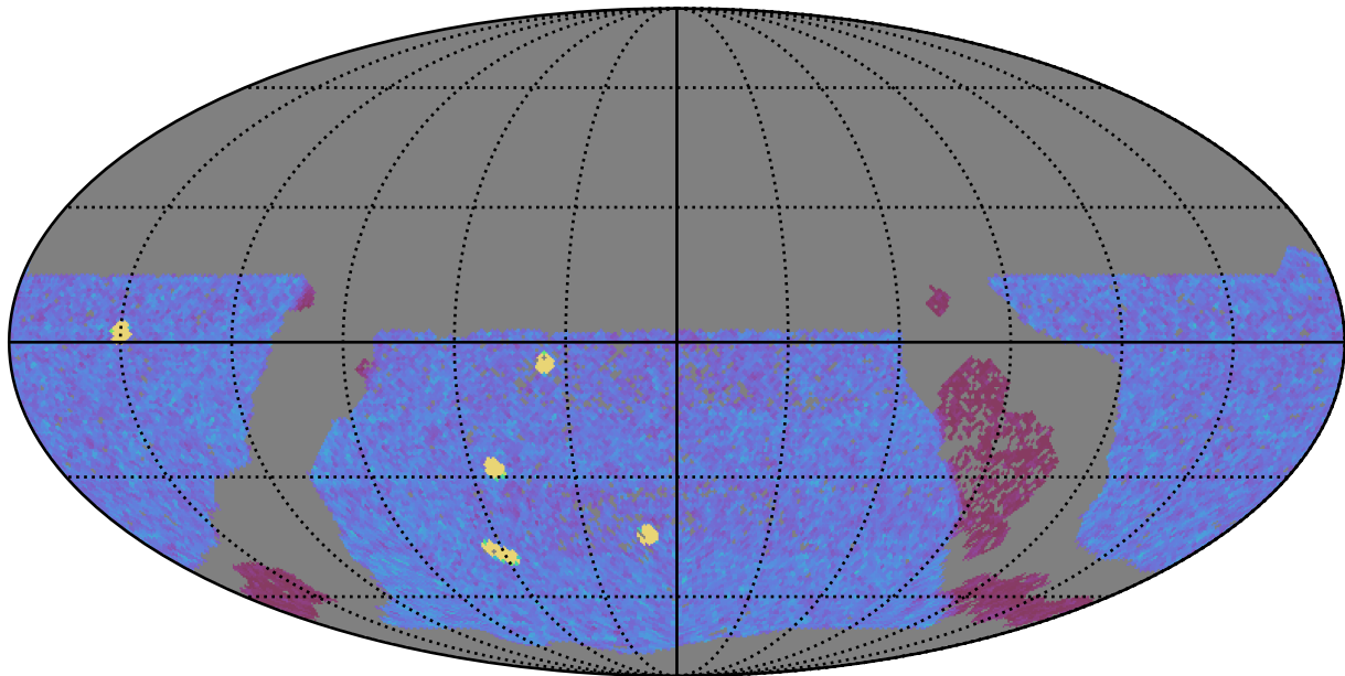
too_elab_heavy_r128_d3_griz_v3.4_10yrs WFD y band: NVisits
