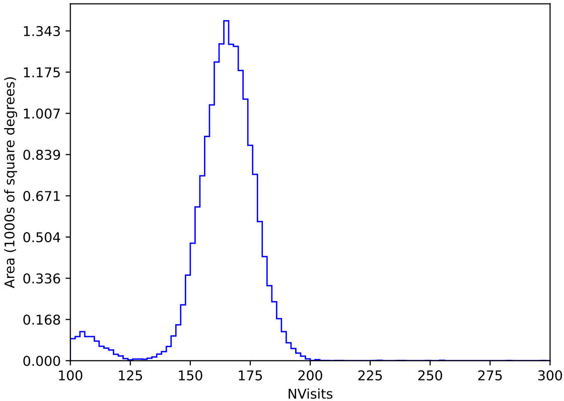
too_elab_heavy_r128_d3_griz_v3.4_10yrs WFD y band: NVisits
