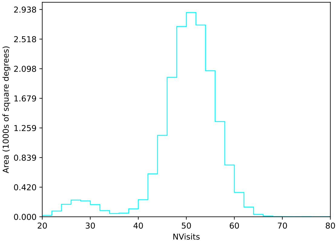
too_elab_heavy_r128_d3_griz_v3.4_10yrs WFD u band: NVisits
