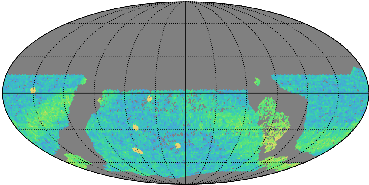
too_elab_heavy_r128_d3_griz_v3.4_10yrs WFD r band: NVisits
