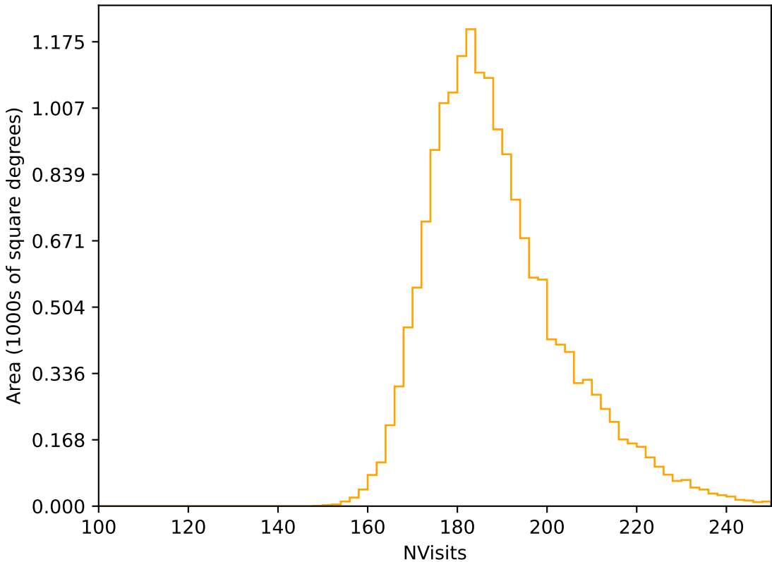
too_elab_heavy_r128_d3_griz_v3.4_10yrs WFD r band: NVisits
