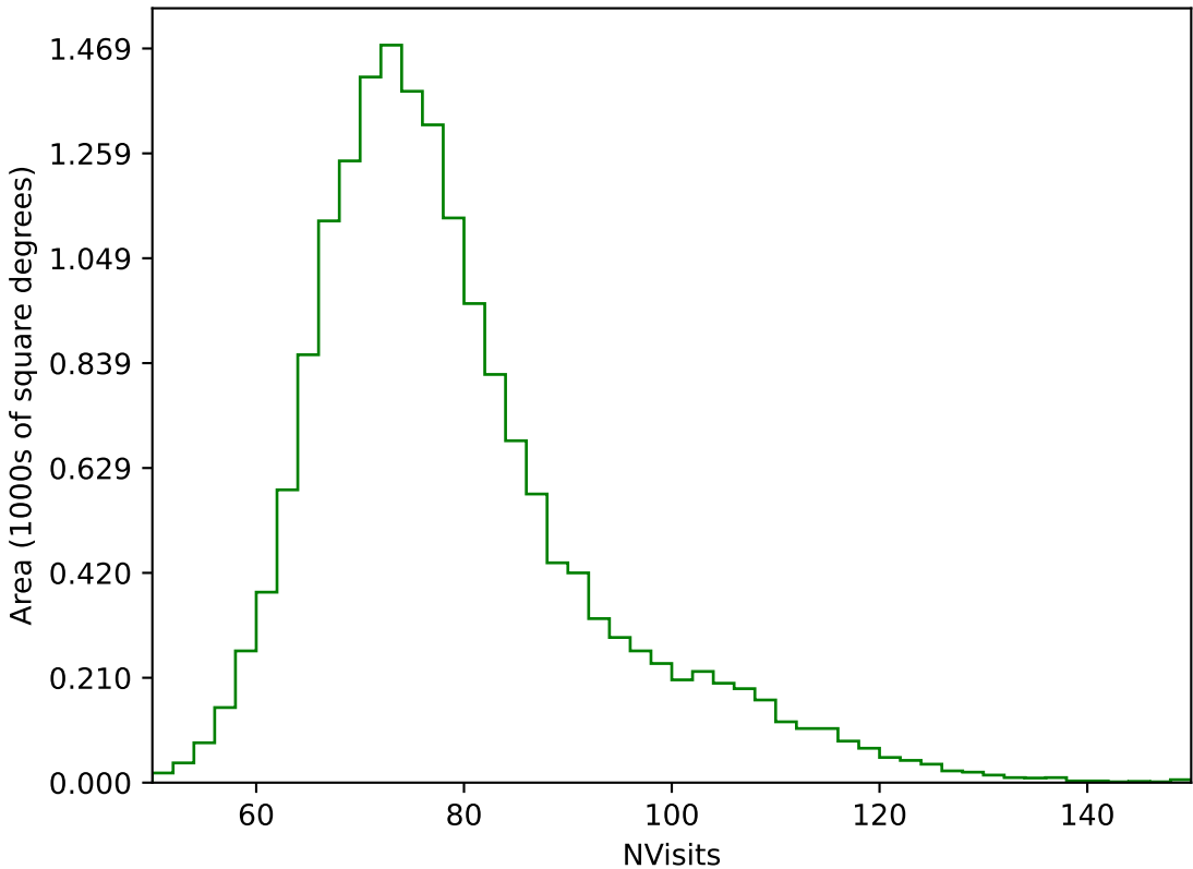
too_elab_heavy_r128_d3_griz_v3.4_10yrs WFD g band: NVisits
