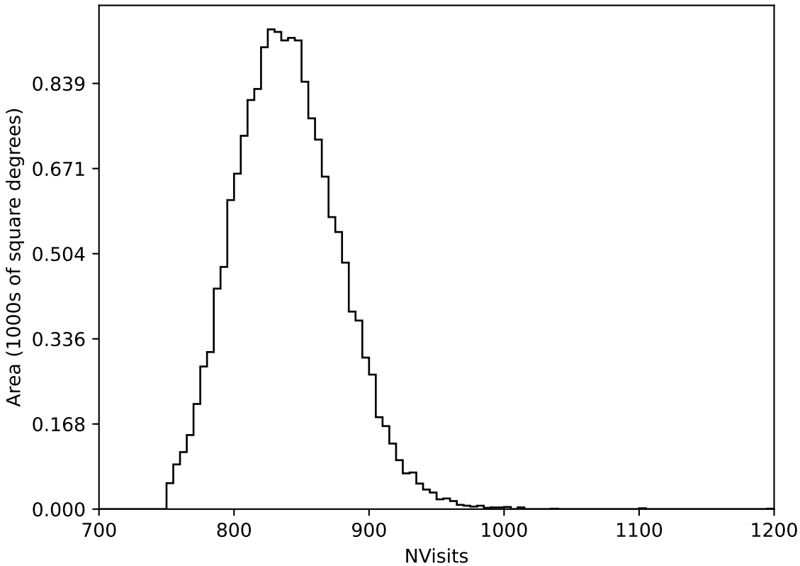
too_elab_heavy_r128_d3_griz_v3.4_10yrs WFD all bands: NVisits
