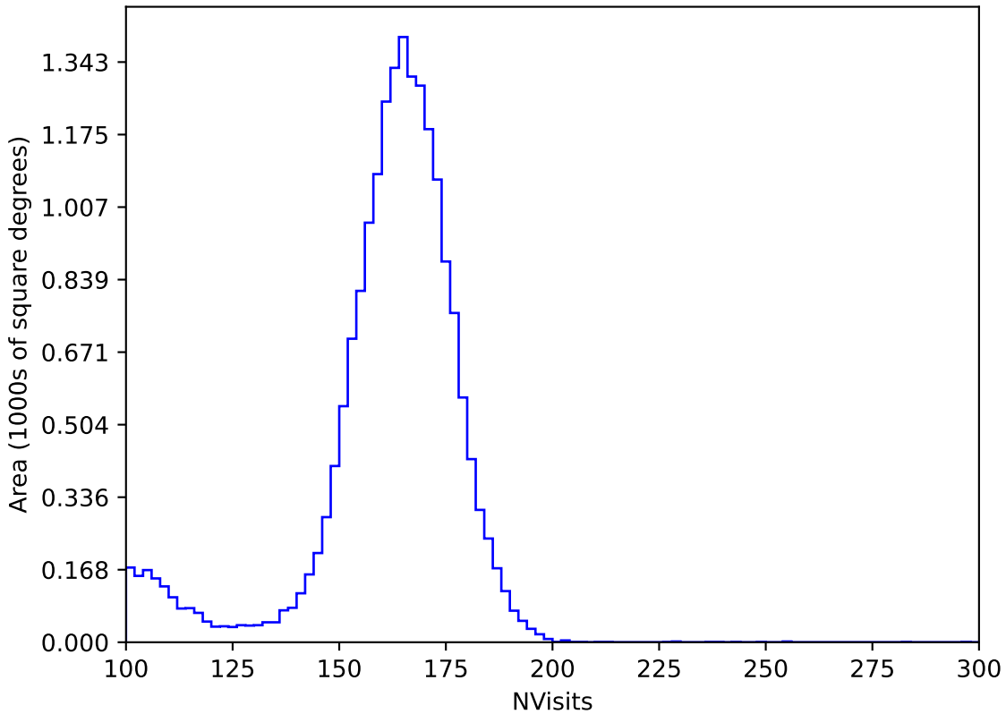
too_elab_heavy_r128_d3_griz_v3.4_10yrs All sky y band: NVisits
