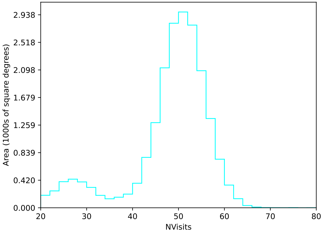
too_elab_heavy_r128_d3_griz_v3.4_10yrs All sky u band: NVisits
