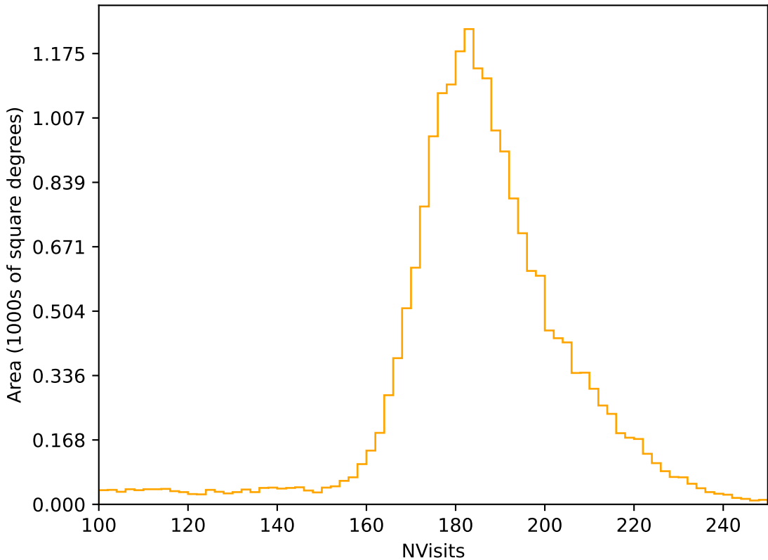
too_elab_heavy_r128_d3_griz_v3.4_10yrs All sky r band: NVisits
