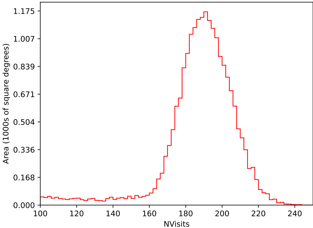
too_elab_heavy_r128_d3_griz_v3.4_10yrs All sky i band: NVisits
