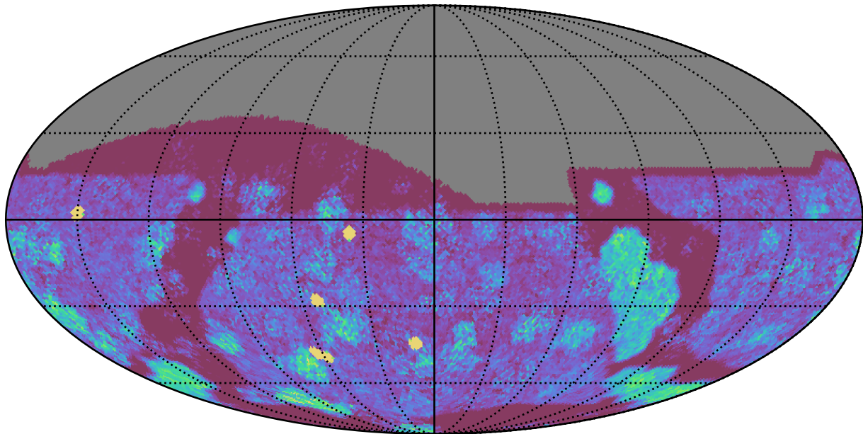
too_elab_heavy_r128_d3_griz_v3.4_10yrs All sky g band: NVisits
