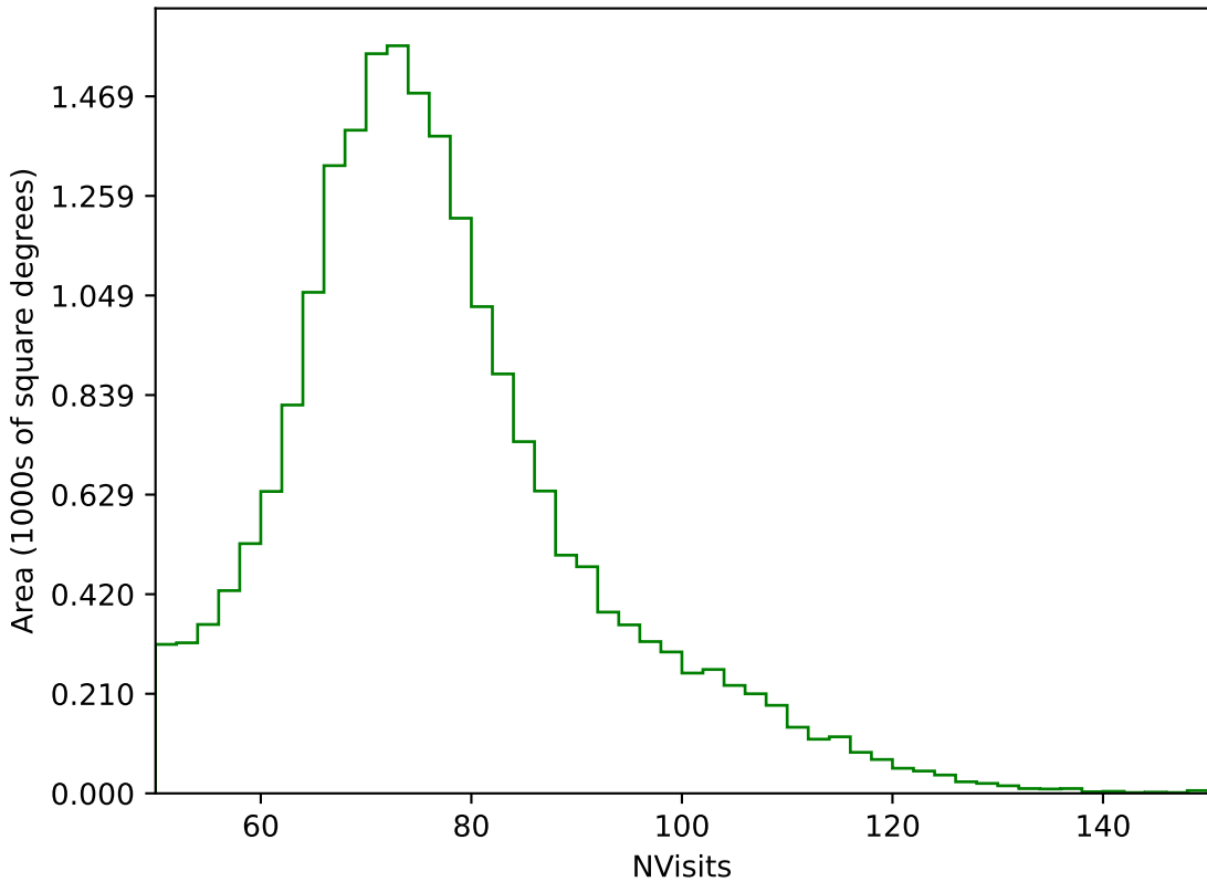
too_elab_heavy_r128_d3_griz_v3.4_10yrs All sky g band: NVisits
