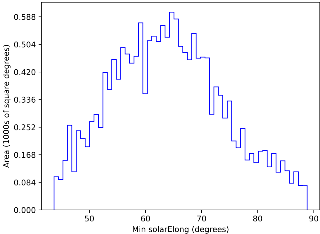
too_elab_heavy_r128_d3_griz_v3.4_10yrs WFD y band: Min solarElong
