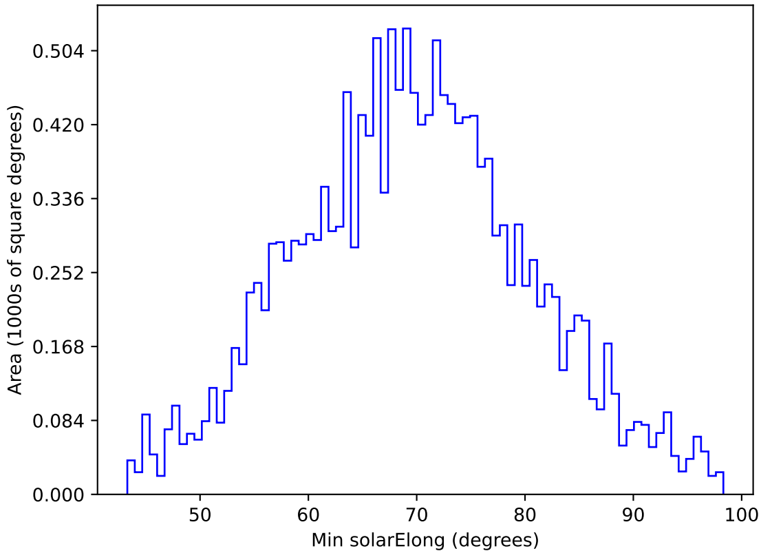
too_elab_heavy_r128_d3_griz_v3.4_10yrs WFD g band: Min solarElong
