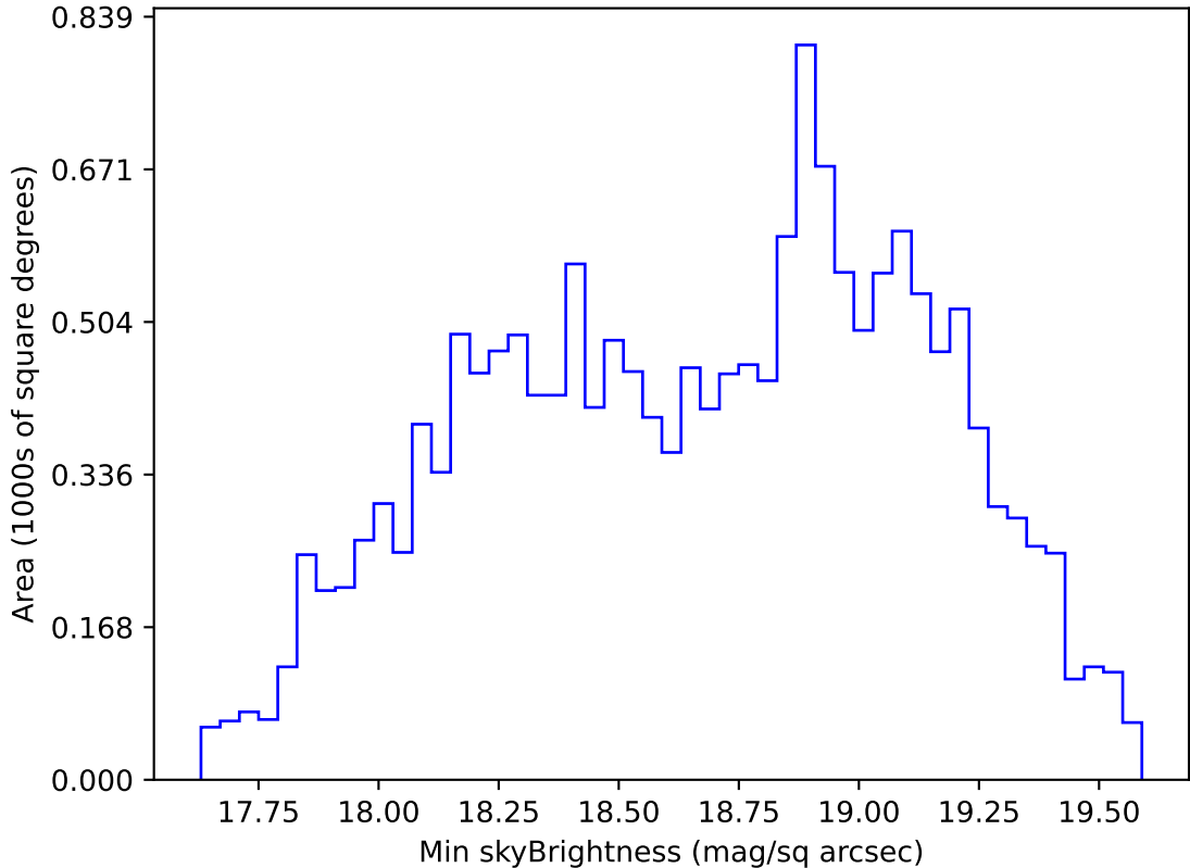
too_elab_heavy_r128_d3_griz_v3.4_10yrs WFD r band: Min skyBrightness
