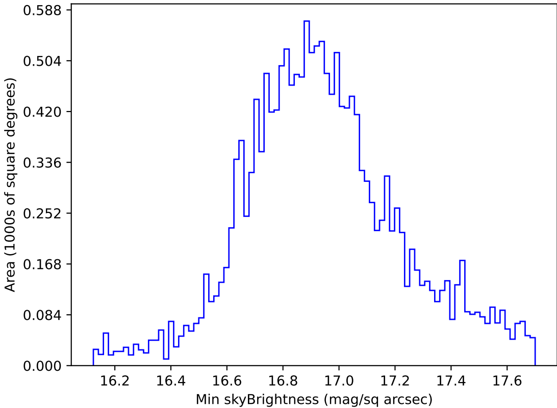
too_elab_heavy_r128_d3_griz_v3.4_10yrs WFD all bands: Min skyBrightness
